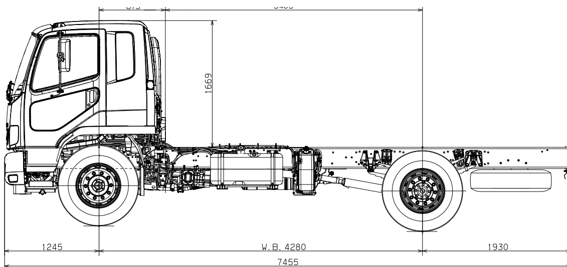
FIGHTER FM1628 – 'H' WHEELBASE
