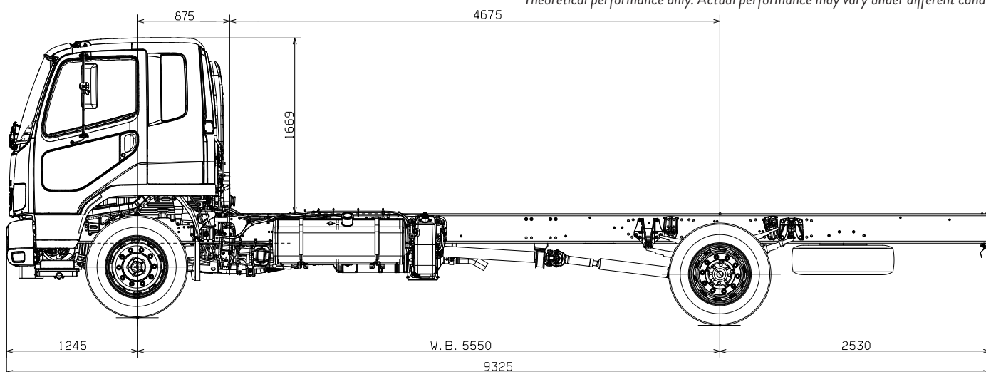
FIGHTER FM1628 – 'M' WHEELBASE
